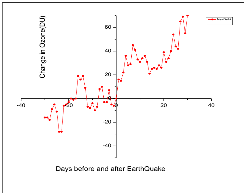
Figure 1: Comparison of change in total ozone (Dobson Units) with respect to the ozone concentration on the earthquake day for Delhi
