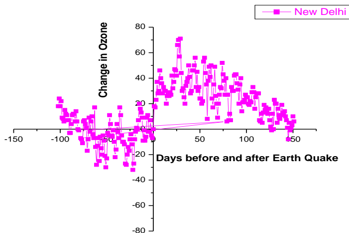
Figure 2: Comparison of change in total ozone (Dobson Units) with respect to the ozone concentration for a period of one year for Delhi
